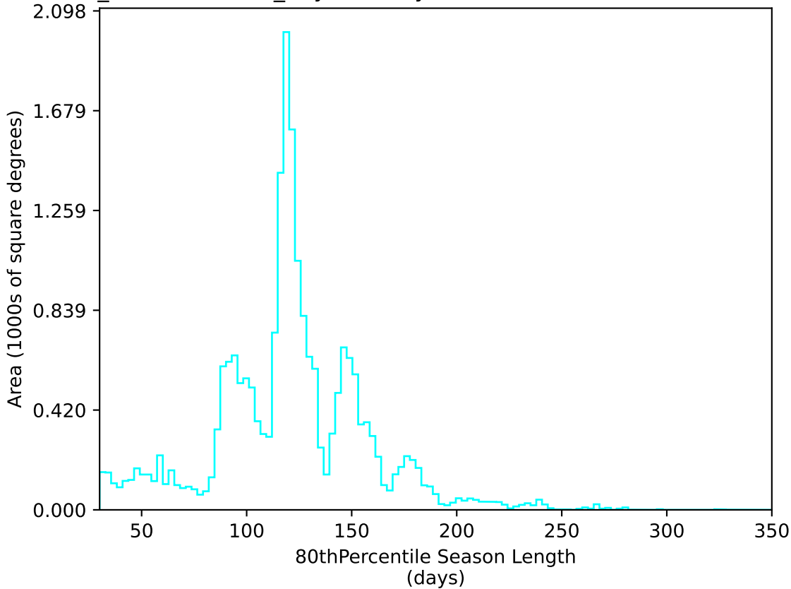
weather_cloudso12v3.4_10yrs All sky u band: 80thPercentile Season Length
