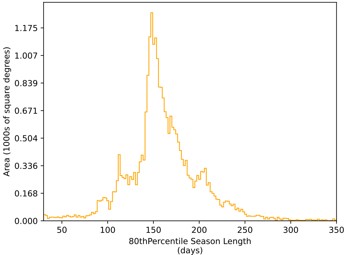
weather_cloudso12v3.4_10yrs All sky r band: 80thPercentile Season Length
