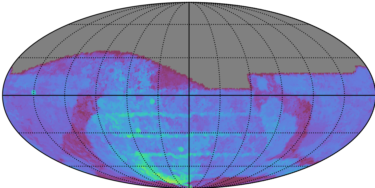
weather_cloudso12v3.4_10yrs All sky g band: 80thPercentile Season Length
