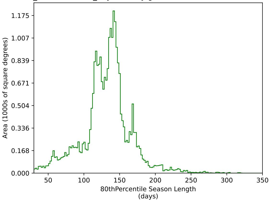
weather_cloudso12v3.4_10yrs All sky g band: 80thPercentile Season Length
