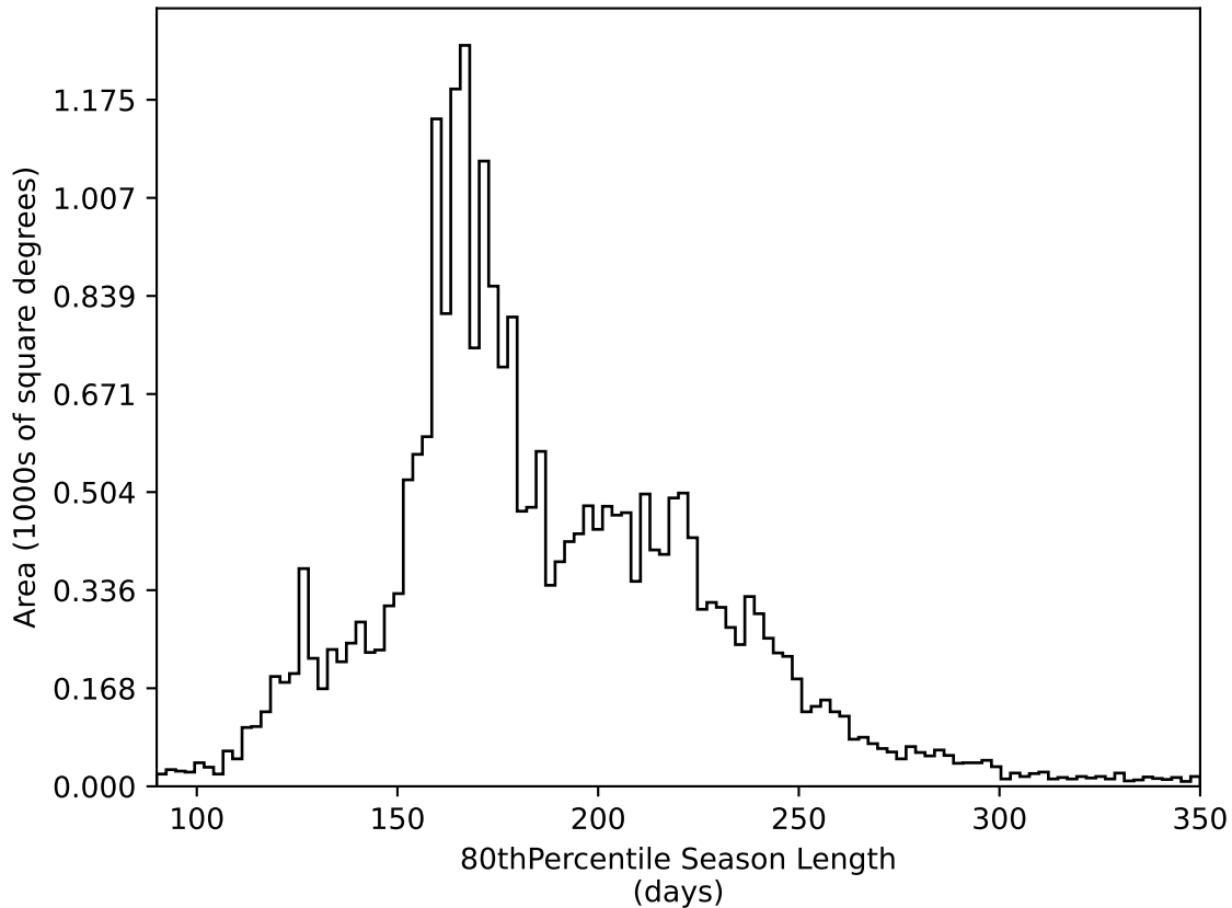
weather_cloudso12v3.4_10yrs All sky all bands: 80thPercentile Season Length
