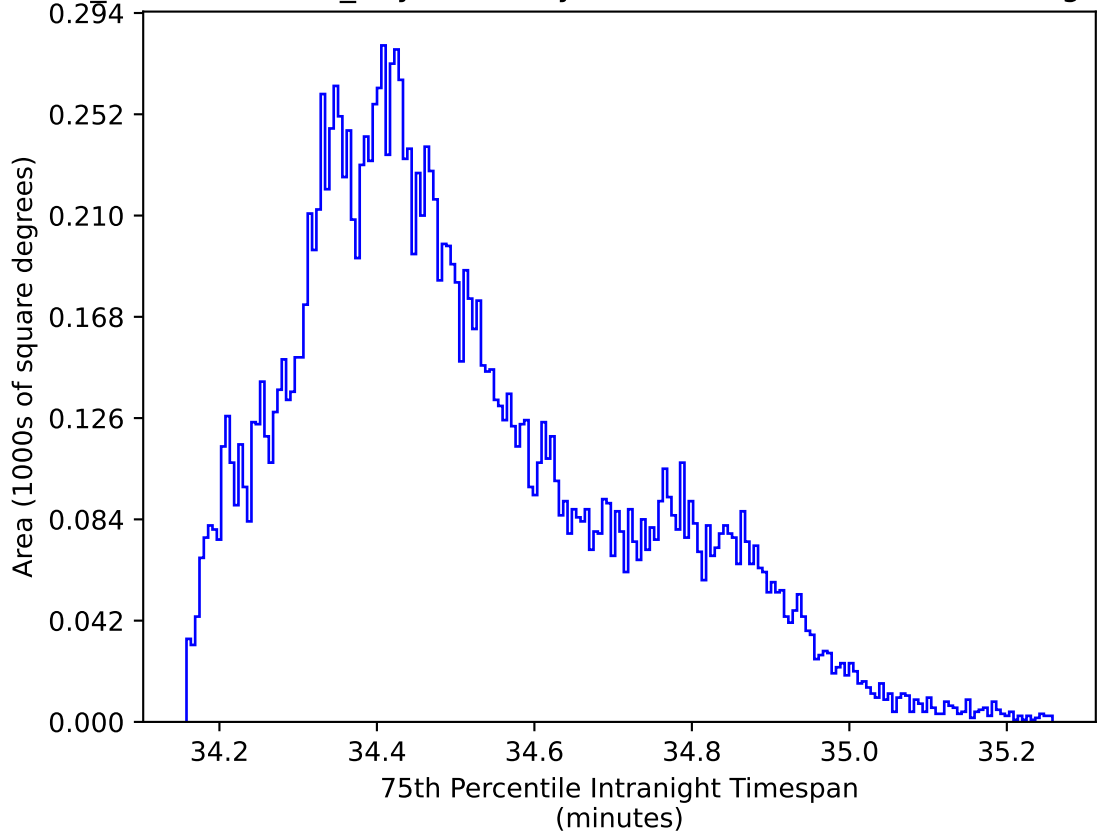
weather_cloudso12v3.4_10yrs WFD zy bands: 75th Percentile Intranight Timespan
