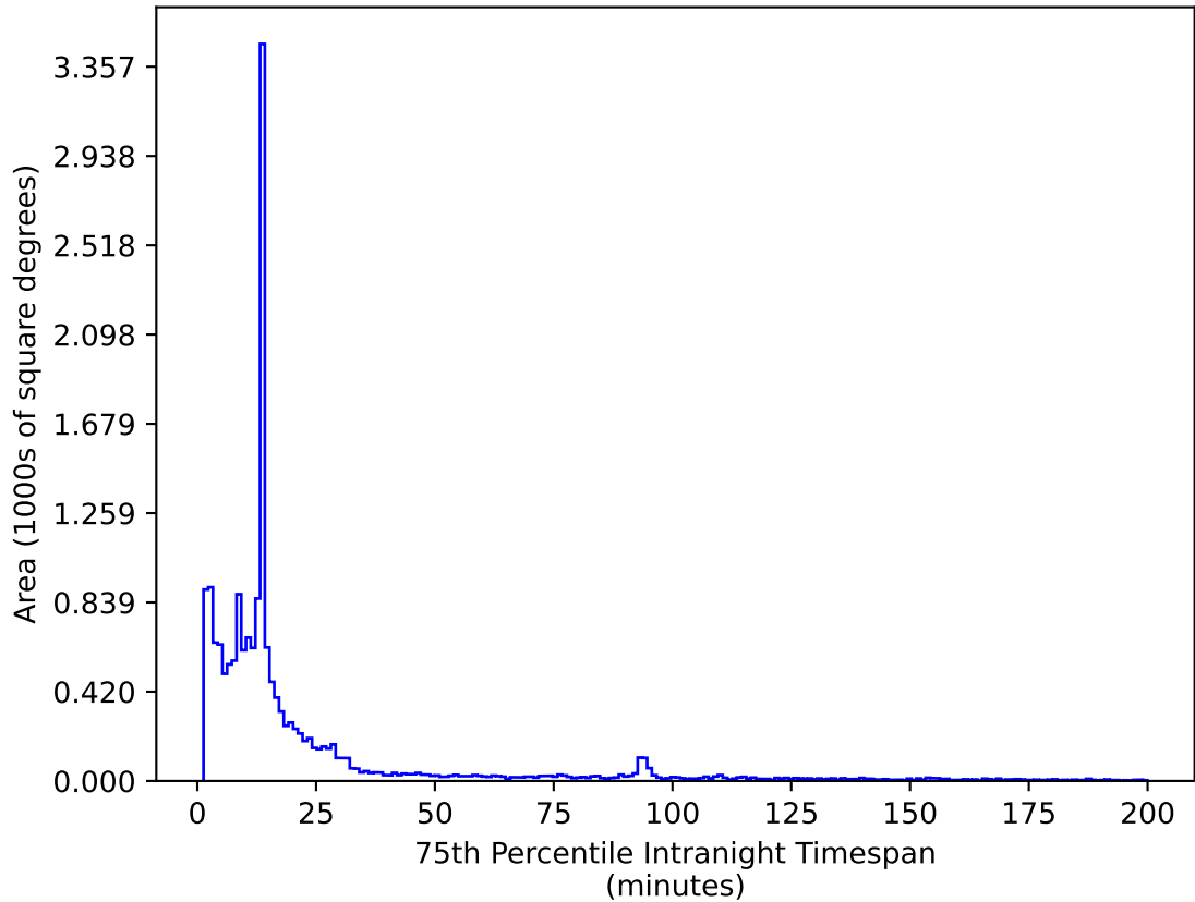
weather_cloudso12v3.4_10yrs WFD z band: 75th Percentile Intranight Timespan
