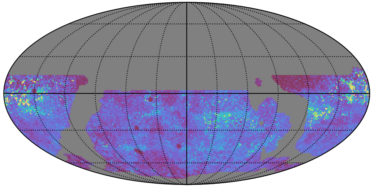
weather_cloudso12v3.4_10yrs WFD y band: 75th Percentile Intranight Timespan
