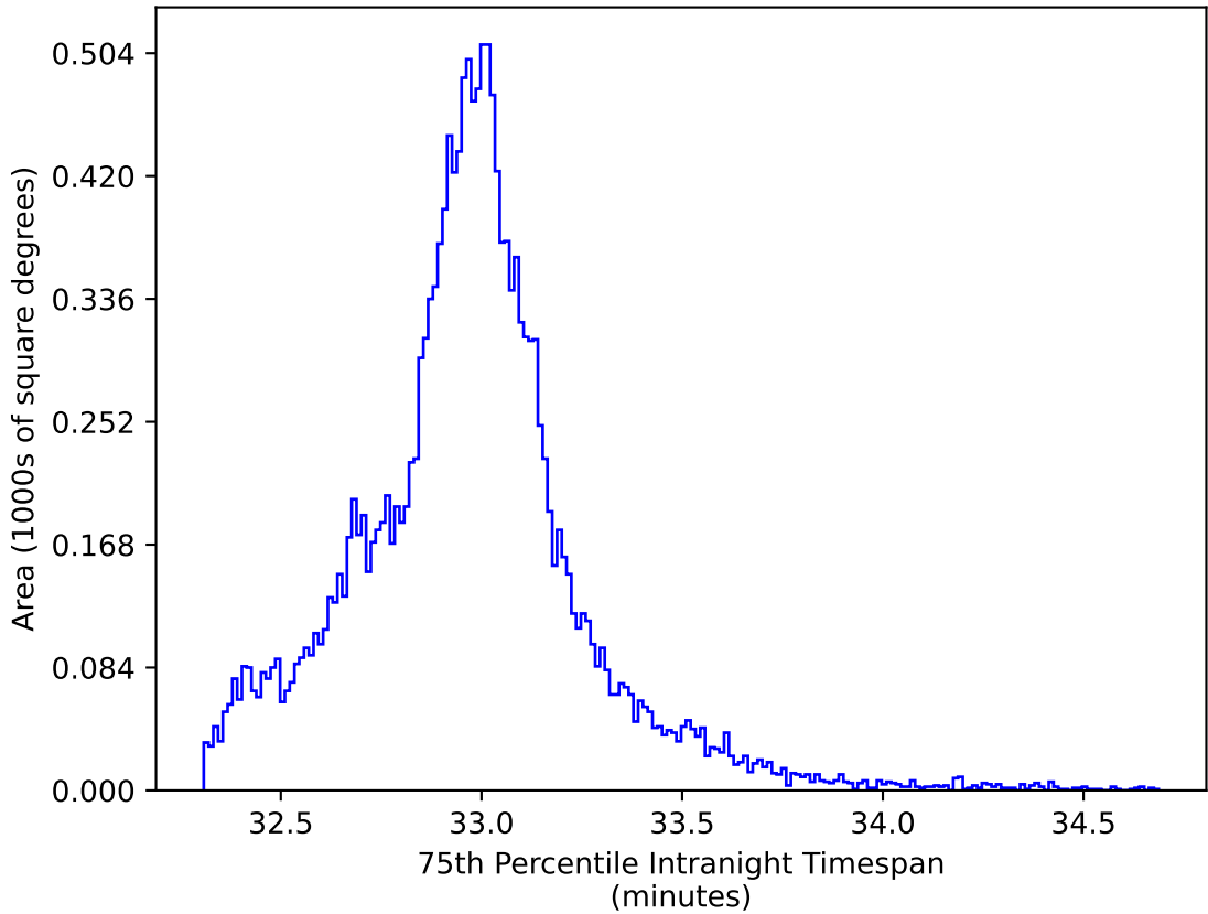
weather_cloudso12v3.4_10yrs WFD y band: 75th Percentile Intranight Timespan
