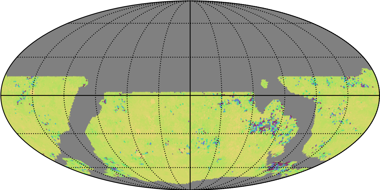
weather_cloudso12v3.4_10yrs WFD ug bands: 75th Percentile Intranight Timespan
