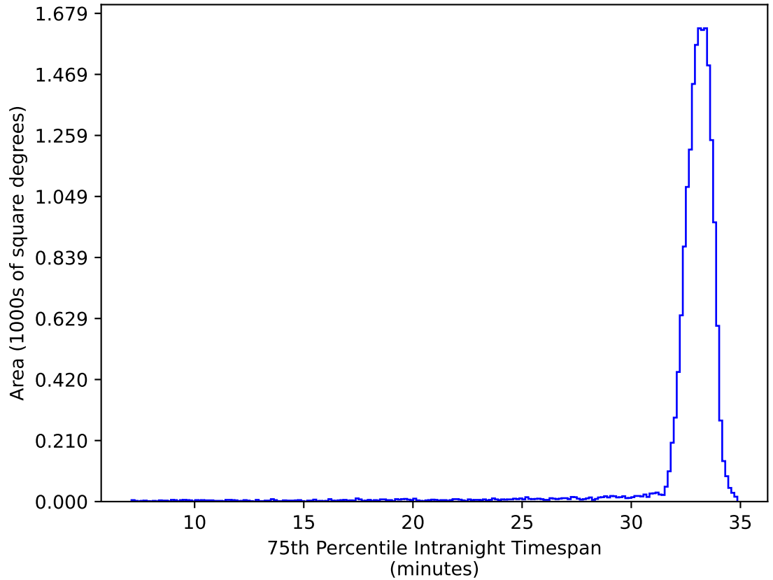
weather_cloudso12v3.4_10yrs WFD ug bands: 75th Percentile Intranight Timespan
