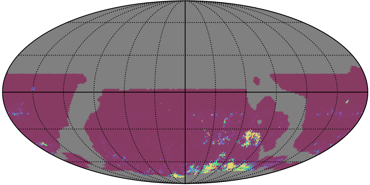
weather_cloudso12v3.4_10yrs WFD ri bands: 75th Percentile Intranight Timespan
