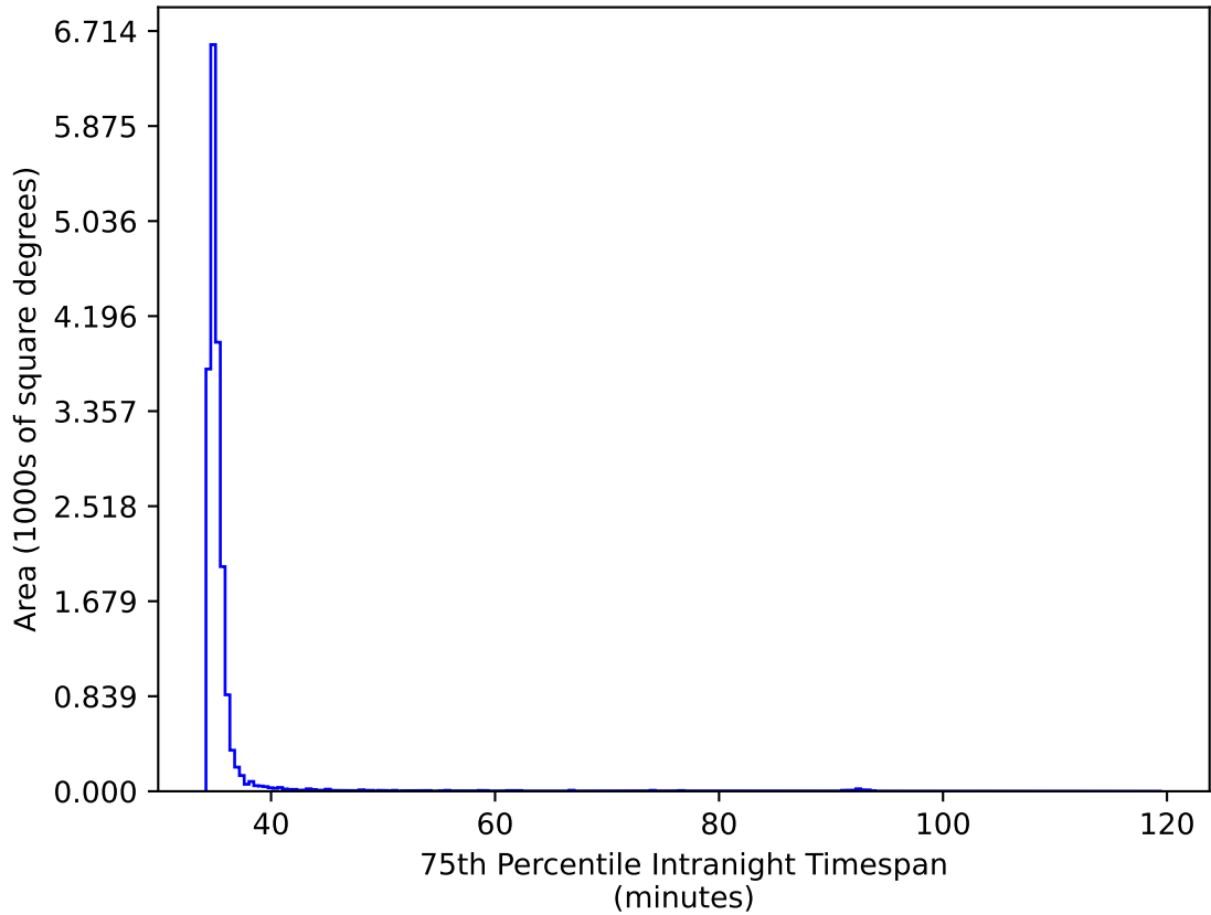
weather_cloudso12v3.4_10yrs WFD ri bands: 75th Percentile Intranight Timespan
