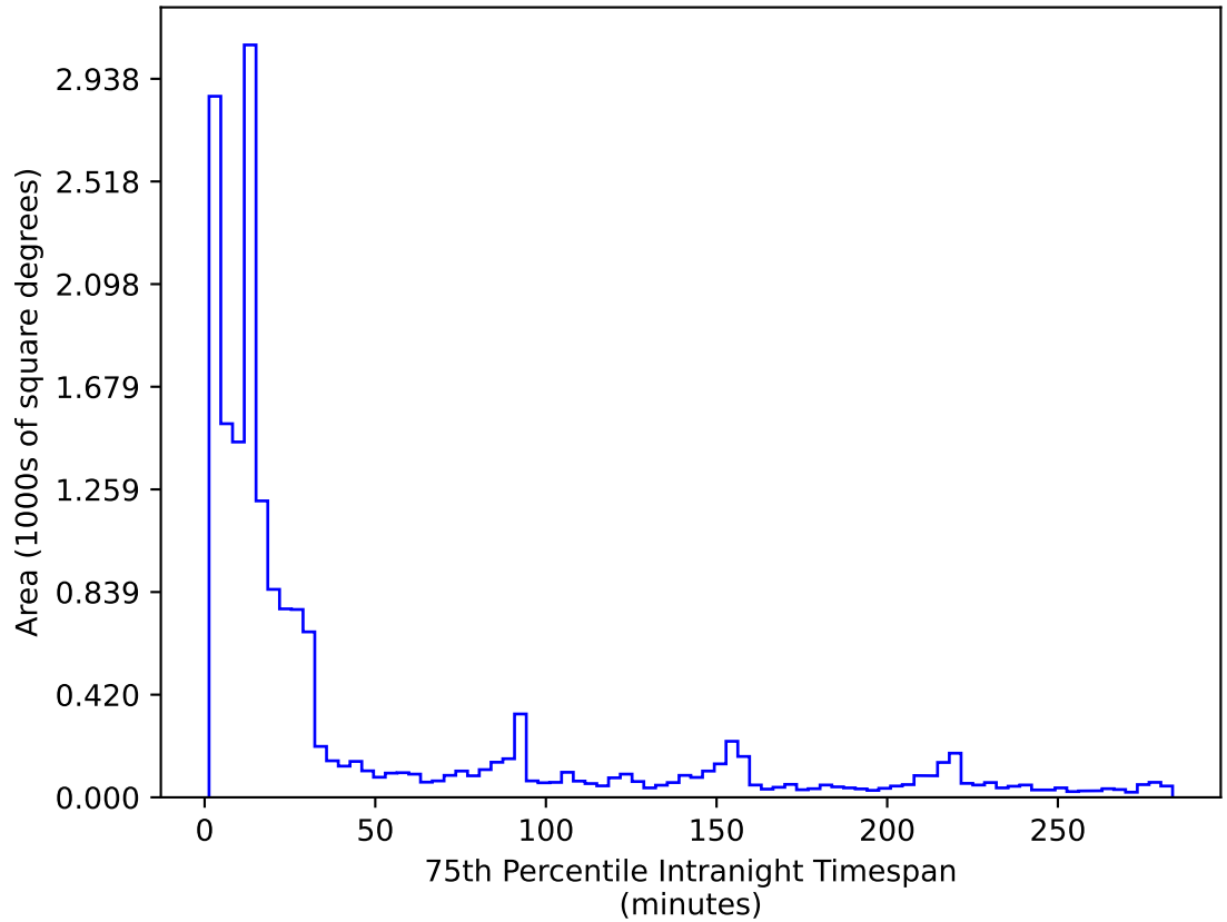
weather_cloudso12v3.4_10yrs WFD r band: 75th Percentile Intranight Timespan
