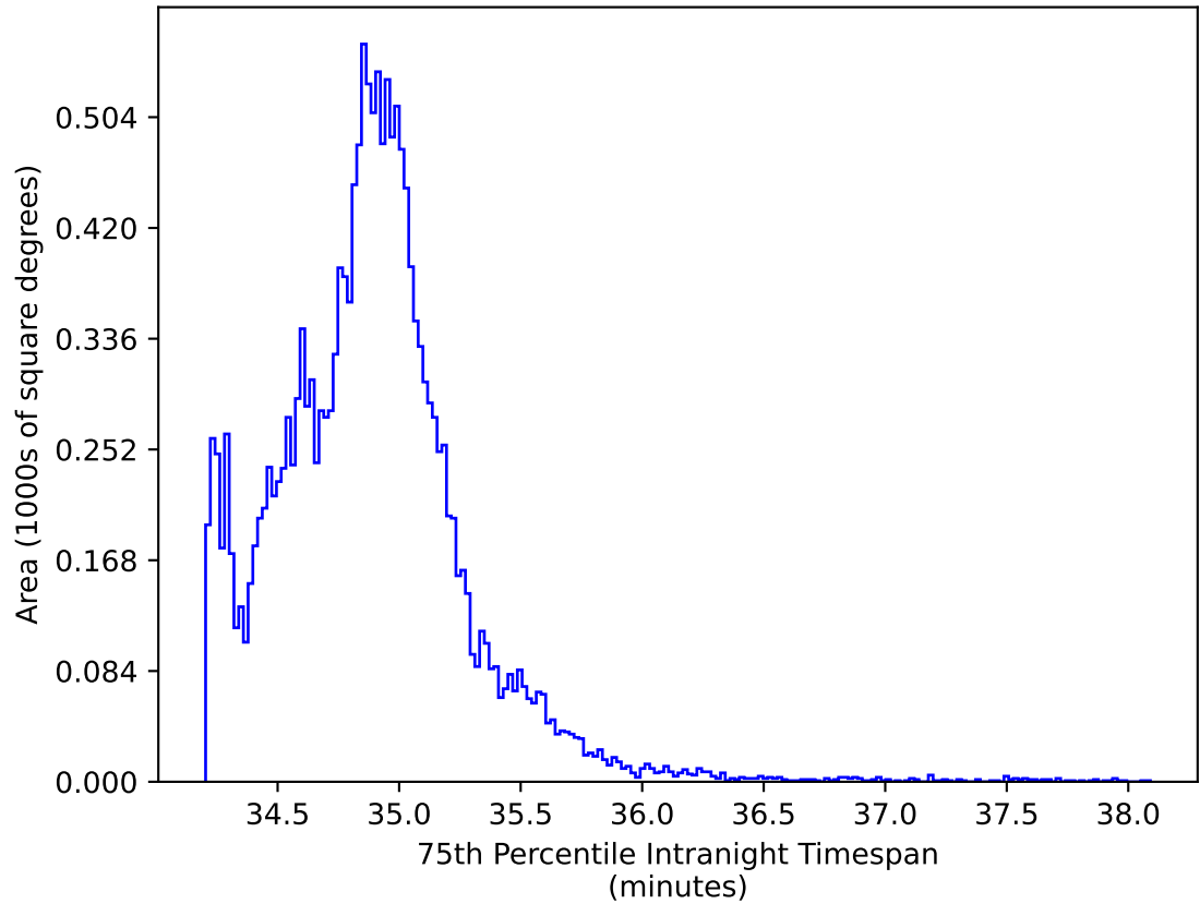
weather_cloudso12v3.4_10yrs WFD iz bands: 75th Percentile Intranight Timespan
