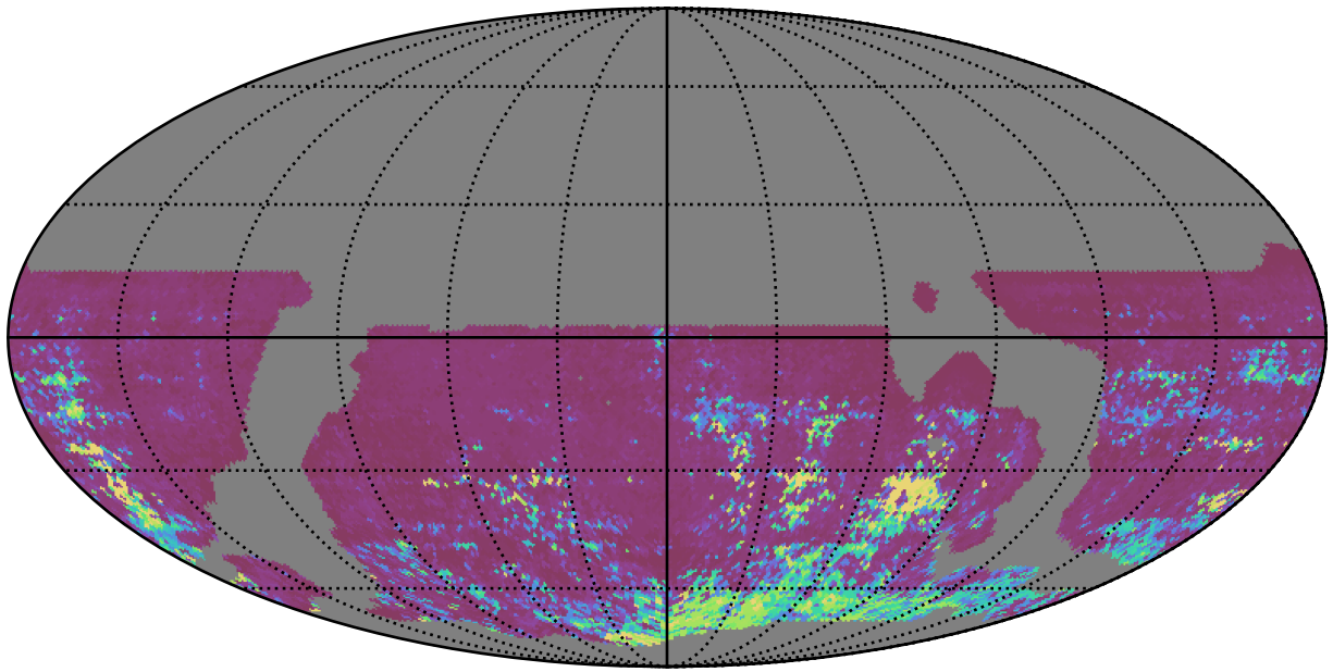
weather_cloudso12v3.4_10yrs WFD i band: 75th Percentile Intranight Timespan
