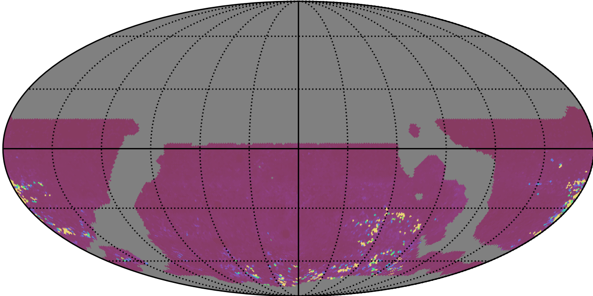
weather_cloudso12v3.4_10yrs WFD gr bands: 75th Percentile Intranight Timespan
