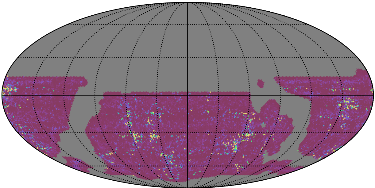
weather_cloudso12v3.4_10yrs WFD g band: 75th Percentile Intranight Timespan
