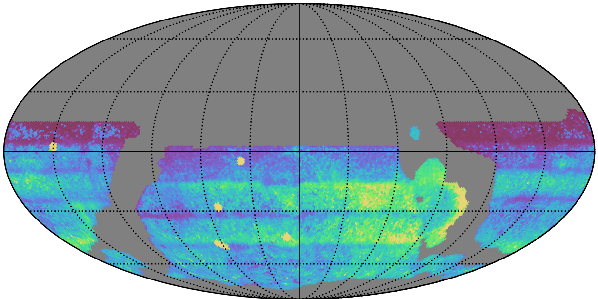
weather_cloudso12v3.4_10yrs WFD all bands: 75th Percentile Intranight Timespan
