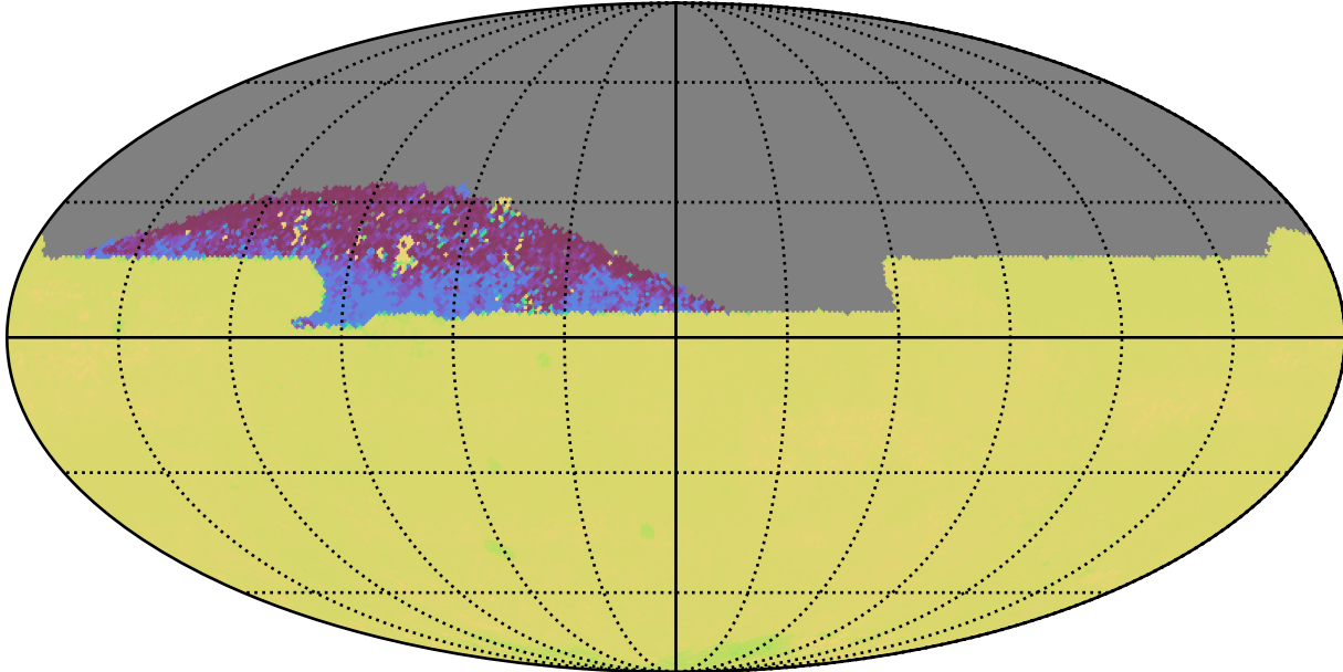
weather_cloudso12v3.4_10yrs All sky zy bands: 75th Percentile Intranight Timespan
