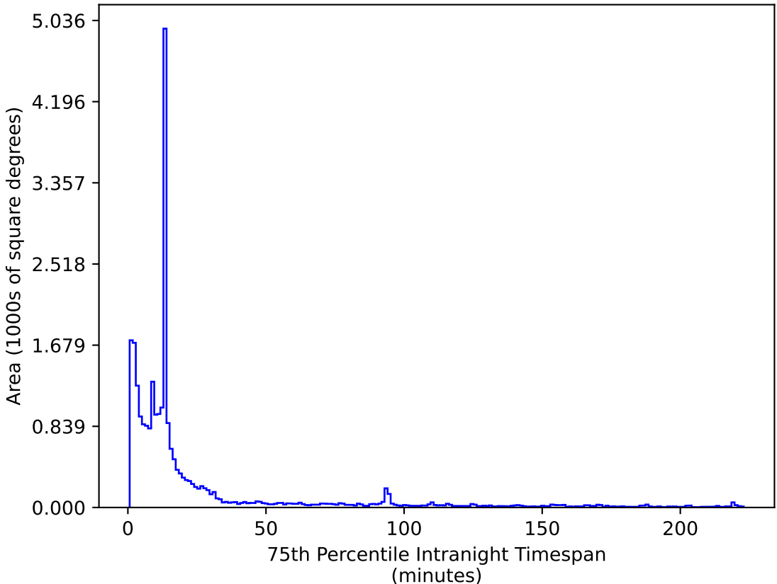
weather_cloudso12v3.4_10yrs All sky z band: 75th Percentile Intranight Timespan
