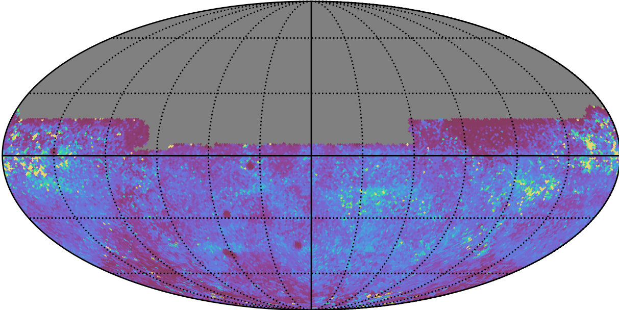
weather_cloudso12v3.4_10yrs All sky y band: 75th Percentile Intranight Timespan
