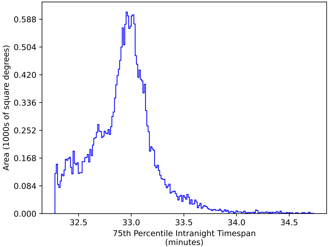
weather_cloudso12v3.4_10yrs All sky y band: 75th Percentile Intranight Timespan
