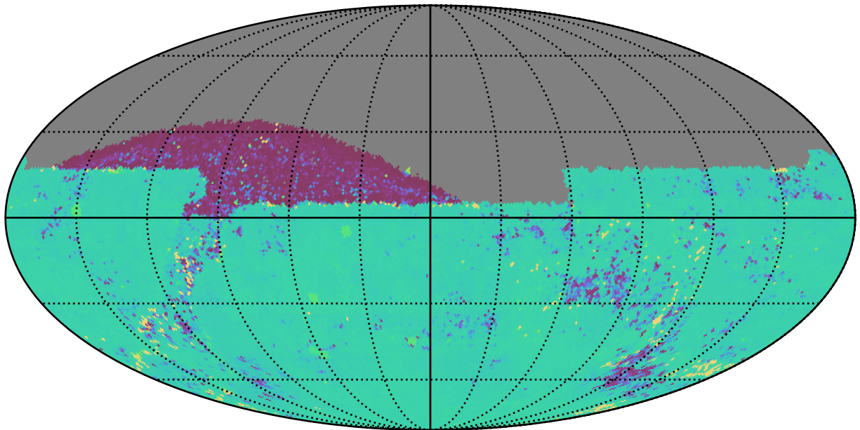
weather_cloudso12v3.4_10yrs All sky ug bands: 75th Percentile Intranight Timespan
