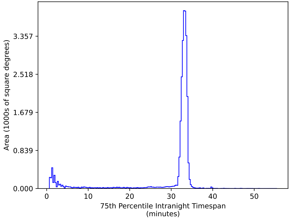
weather_cloudso12v3.4_10yrs All sky ug bands: 75th Percentile Intranight Timespan
