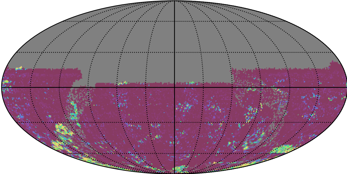
weather_cloudso12v3.4_10yrs All sky u band: 75th Percentile Intranight Timespan
