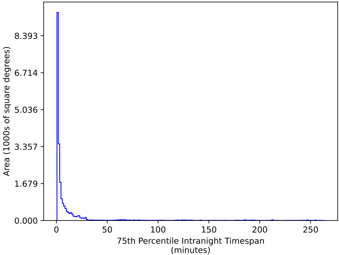
weather_cloudso12v3.4_10yrs All sky u band: 75th Percentile Intranight Timespan
