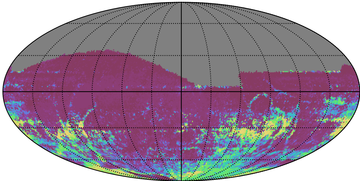
weather_cloudso12v3.4_10yrs All sky r band: 75th Percentile Intranight Timespan
