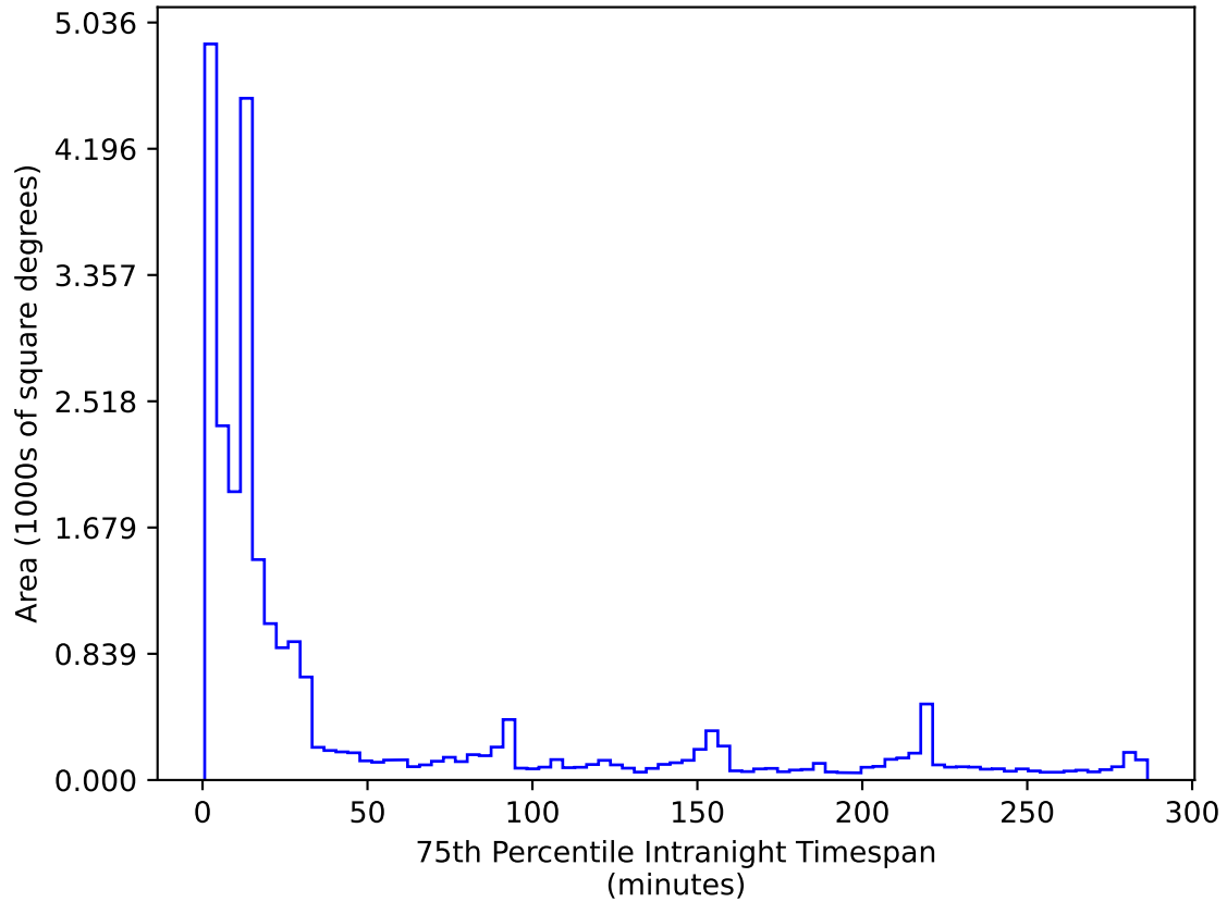
weather_cloudso12v3.4_10yrs All sky r band: 75th Percentile Intranight Timespan
