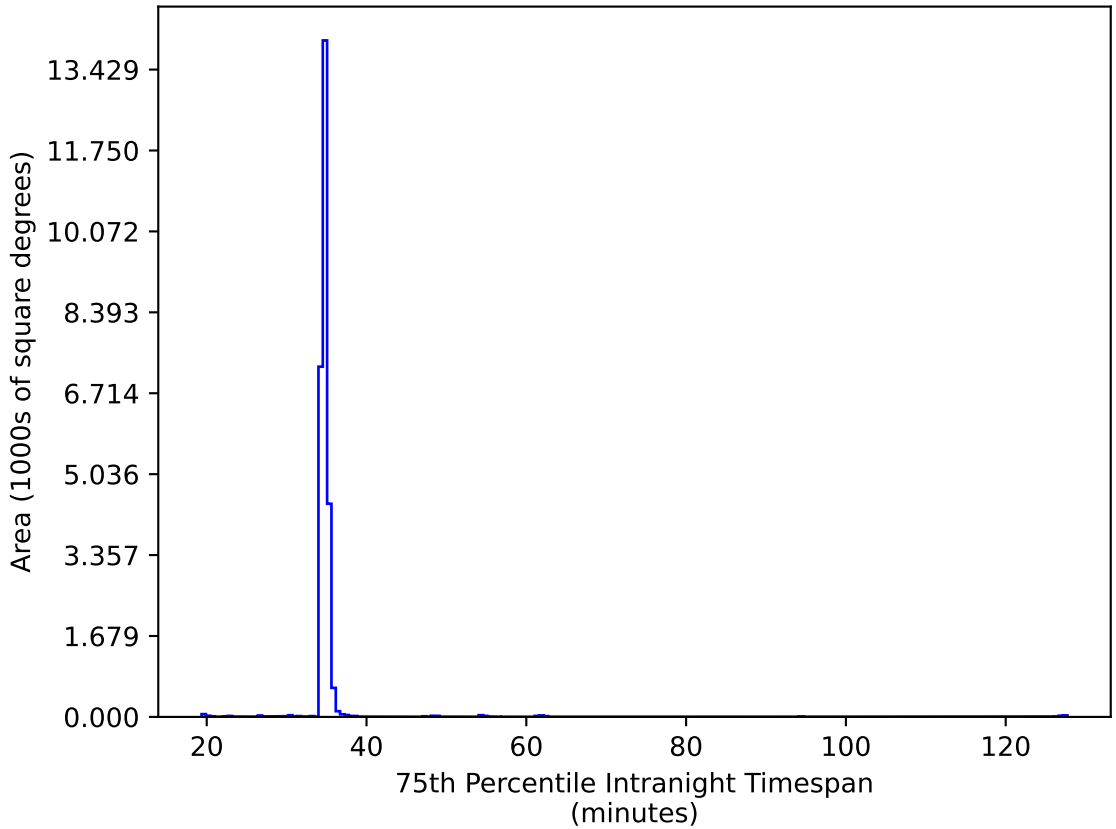
weather_cloudso12v3.4_10yrs All sky iz bands: 75th Percentile Intranight Timespan
