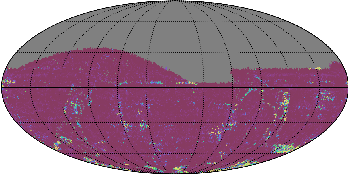
weather_cloudso12v3.4_10yrs All sky g band: 75th Percentile Intranight Timespan
