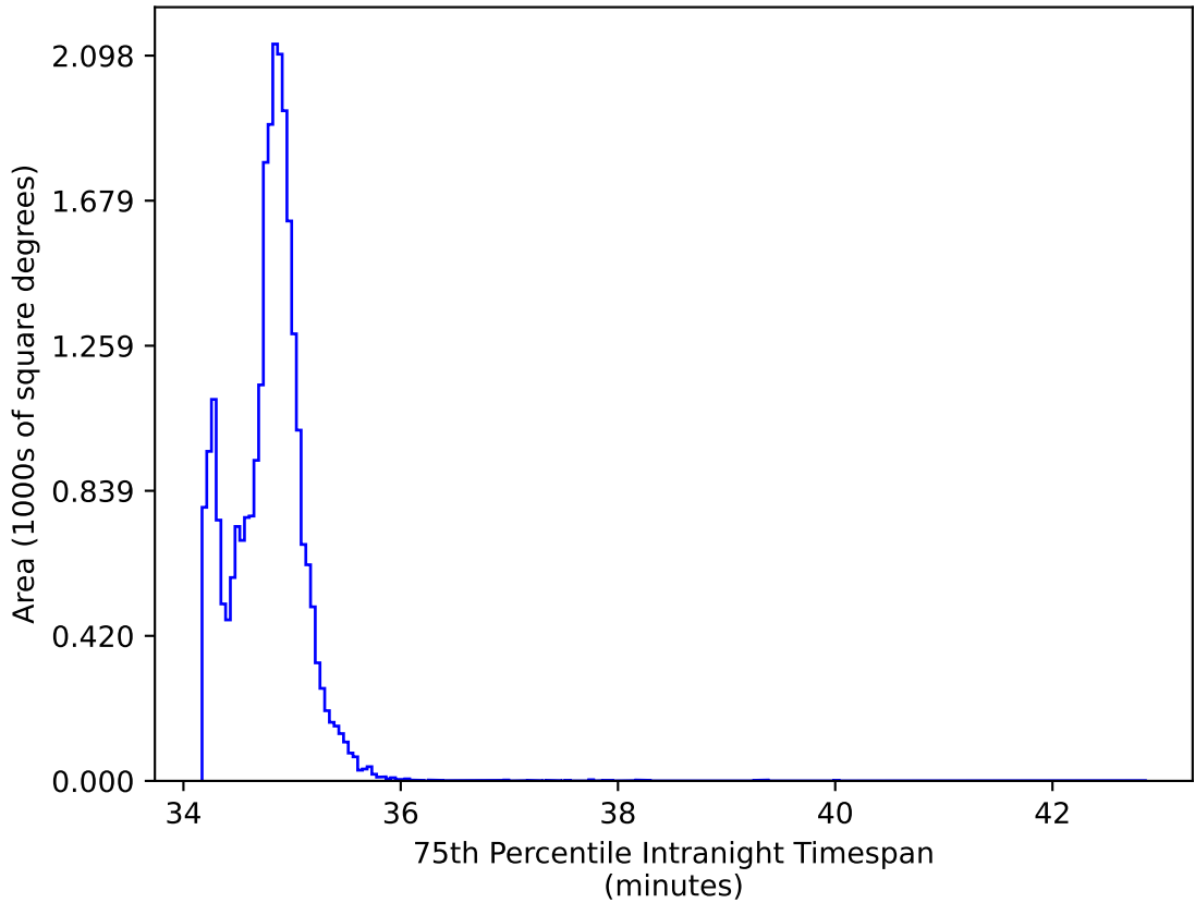
weather_cloudso12v3.4_10yrs All sky all bands: 75th Percentile Intranight Timespan
