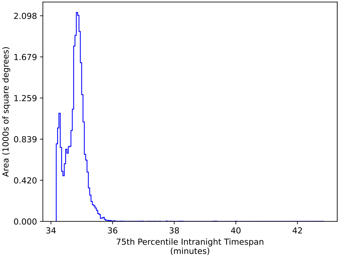
weather_cloudso12v3.4_10yrs All sky: 75th Percentile Intranight Timespan
