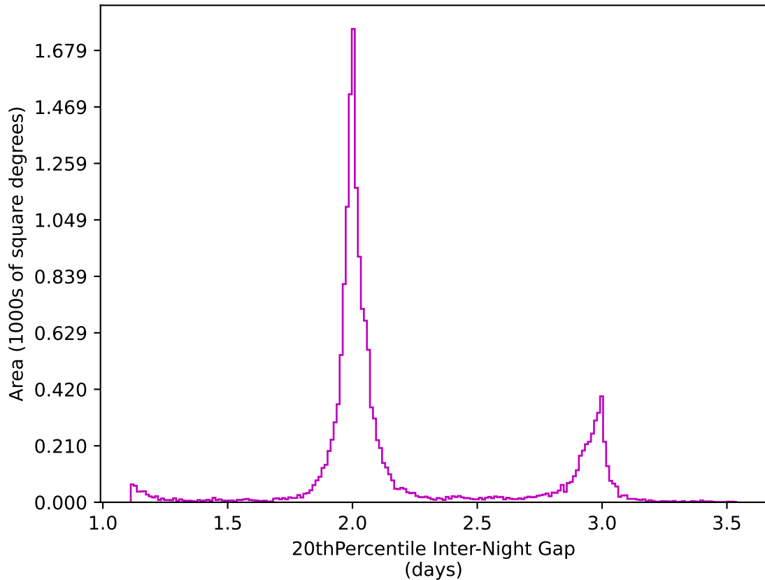
weather_cloudso12v3.4_10yrs WFD z band: 20thPercentile Inter-Night Gap
