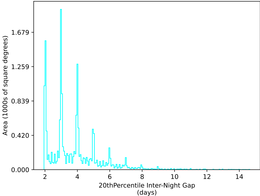
weather_cloudso12v3.4_10yrs WFD u band: 20thPercentile Inter-Night Gap
