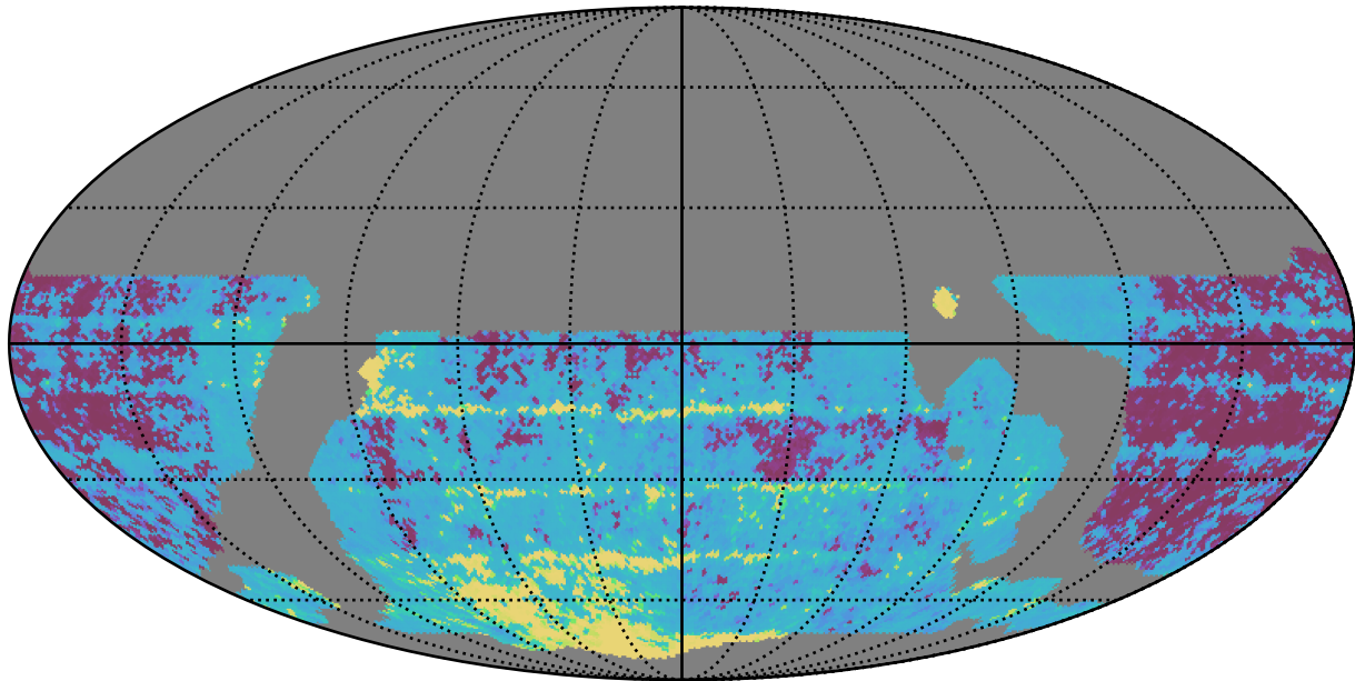
weather_cloudso12v3.4_10yrs WFD r band: 20thPercentile Inter-Night Gap
