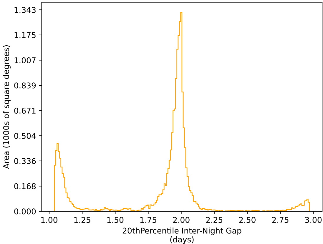
weather_cloudso12v3.4_10yrs WFD r band: 20thPercentile Inter-Night Gap
