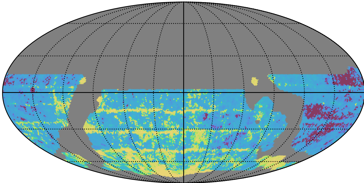
weather_cloudso12v3.4_10yrs WFD i band: 20thPercentile Inter-Night Gap
