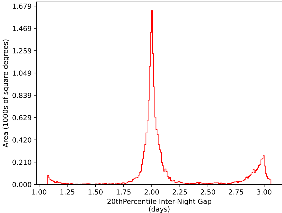
weather_cloudso12v3.4_10yrs WFD i band: 20thPercentile Inter-Night Gap
