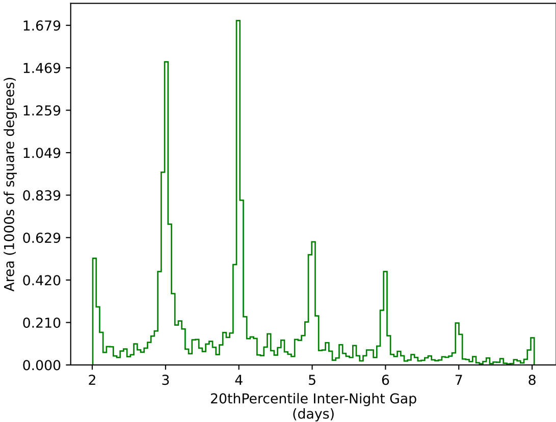
weather_cloudso12v3.4_10yrs WFD g band: 20thPercentile Inter-Night Gap
