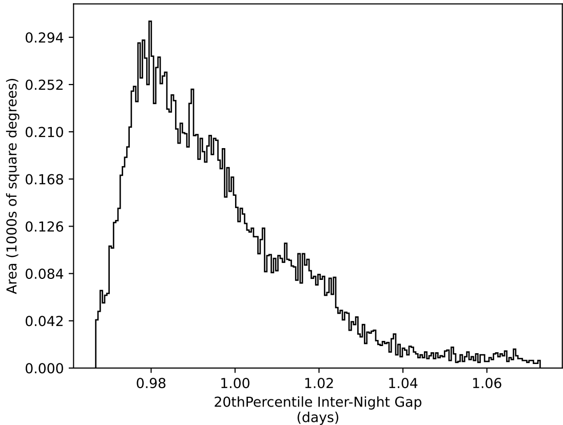
weather_cloudso12v3.4_10yrs WFD all bands: 20thPercentile Inter-Night Gap
