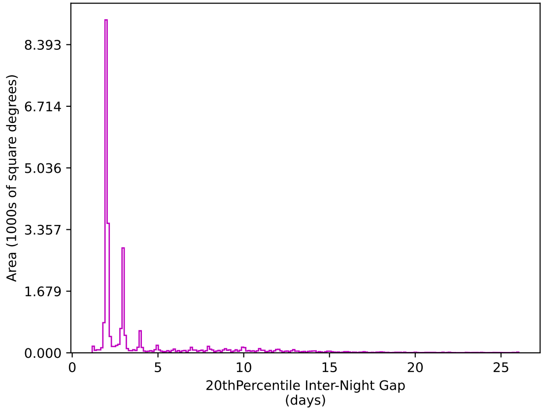
weather_cloudso12v3.4_10yrs All sky z band: 20thPercentile Inter-Night Gap
