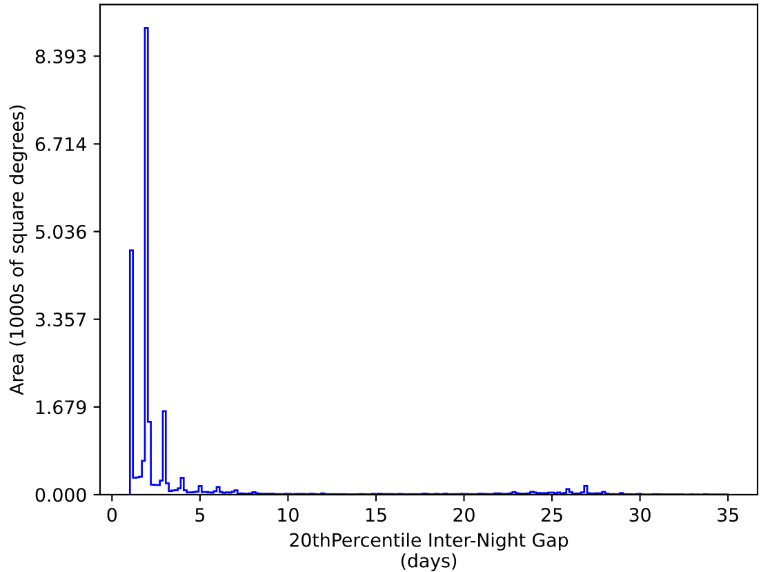
weather_cloudso12v3.4_10yrs All sky y band: 20thPercentile Inter-Night Gap
