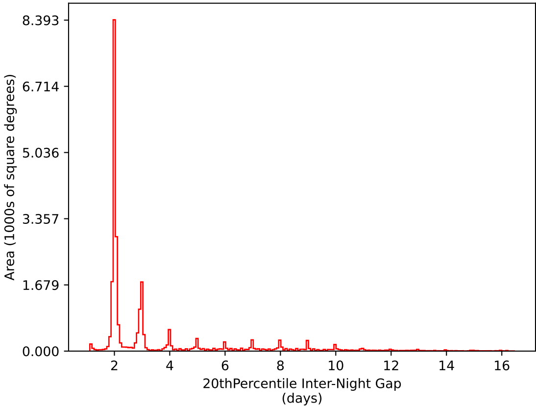
weather_cloudso12v3.4_10yrs All sky i band: 20thPercentile Inter-Night Gap
