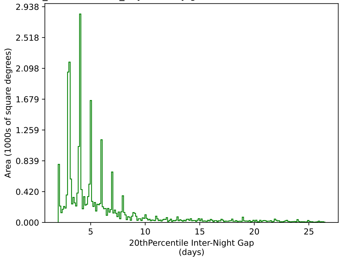
weather_cloudso12v3.4_10yrs All sky g band: 20thPercentile Inter-Night Gap
