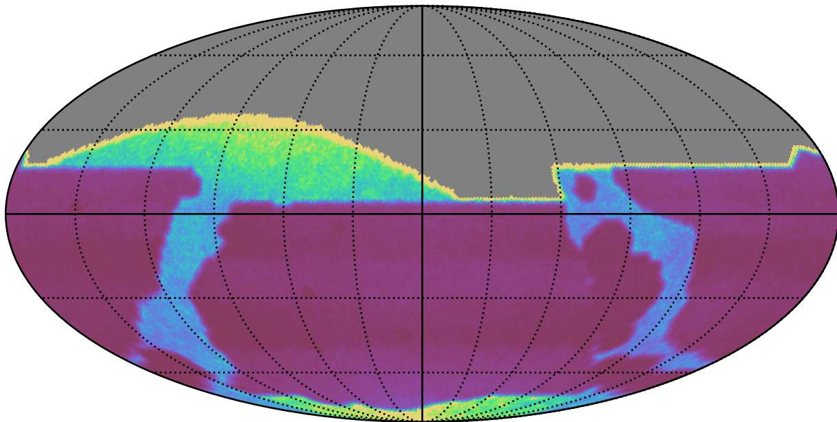
weather_cloudso12v3.4_10yrs : properMotion
