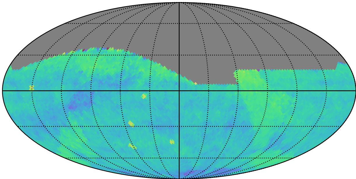
weather_cloudso12v3.4_10yrs (g or r or i): PairFraction
