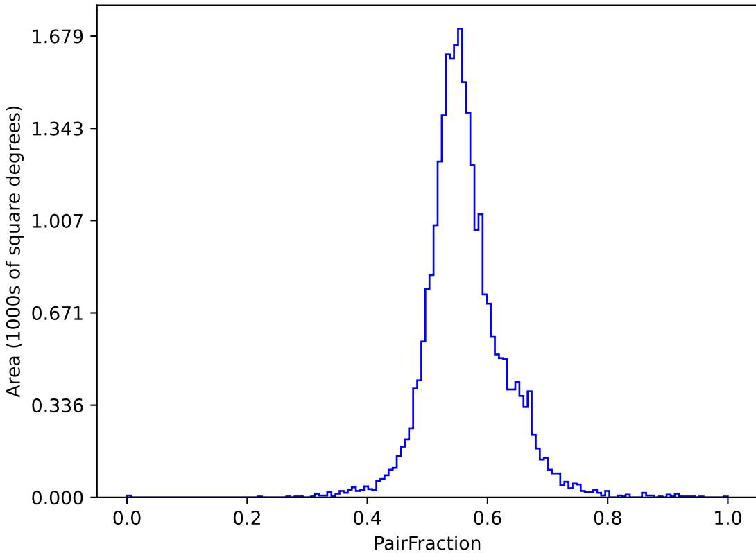
weather_cloudso12v3.4_10yrs (g or r or i): PairFraction
