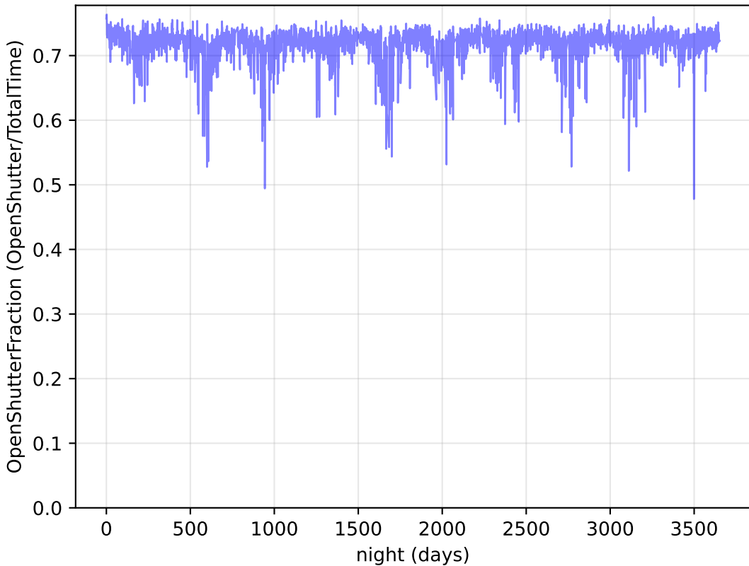
weather_cloudso12v3.4_10yrs : OpenShutterFraction
