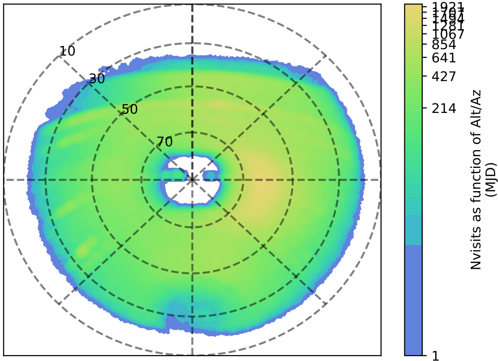
weather_cloudso12v3.4_10yrs y: Nvisits as function of Alt/Az
